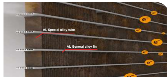
Toshiba aluminum heat exchanger
